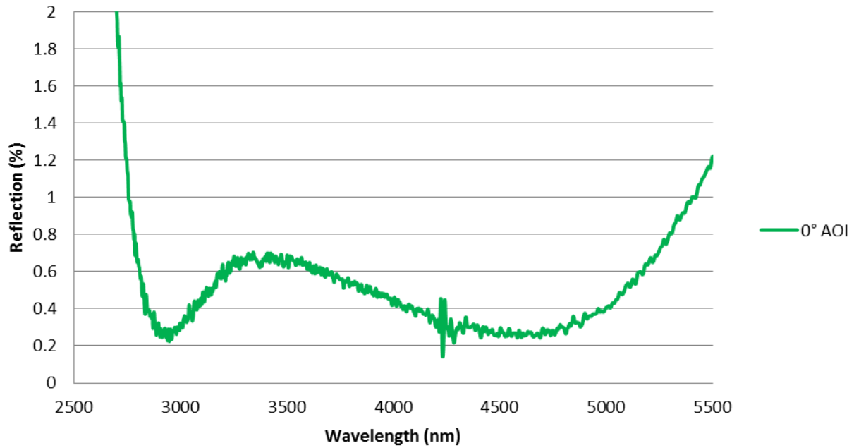
Si PBS Cube, Scan of AR Coated Surface
